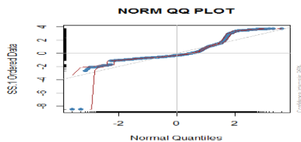
Fig 11 PDS/NGN Normal Q-Q plot
