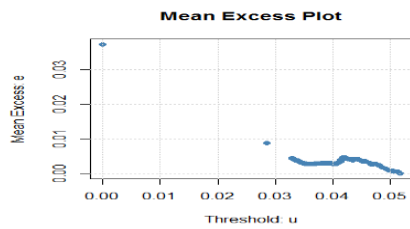
Fig 3 DAN/NGN mean excess plot
